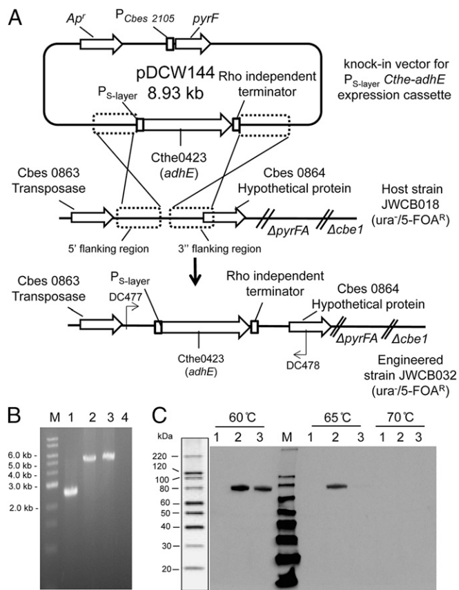
Fig. 3. Targeted insertion and expression of the C. thermocellum ATCC27405 adhE gene ( Cthe0423 ) in C. bescii . (A) A diagram of the integration vector pDCW144 (Fig. S2), which contains the P_{S-layer} - Cthe-adhE expression cassette and pyrF cassette (30) for selection of transformants. Homologous recombination can occur at the upstream- or downstream-targeted chromosomal regions, integrating the plasmid into the genome and generating a strain that is a uracil prototroph. Counter selection with 5-FOA selects for loss of the plasmid sequences but not the adhE expression cassette. Bent arrows depict primers used for verification of the integrated expression cassette (2.6 kb). Ap^R , apramycin resistance gene cassette. (B) Gel depicting PCR products amplified from the targeted chromosome region in JWCB018 ( ldh - , lane 1), JWCB032 ( ldh - adhE + , lane 2), and JWCB032 [ ldh - adhE (EA) + , lane 3] amplified by primers DC477 and DC478. M: 1-kb DNA ladder (New England Biolabs). (C) Western blot analysis of C. bescii strains used in this study. The 77 \mu g of total cell protein lysate isolated from the mid-log-phase cultures grown at various temperatures, either 60 °C, 65 °C, or 70 °C, were electrophoresed and probed with His-tag antibody as described in Methods . Lane 1, ldh - ; lane 2, ldh - adhE + ; lane 3, ldh - adhE (EA) + ; M, MagicMark XP Western Protein Standard (Invitrogen).
